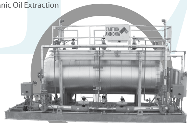
Anhydrous ammonia unloading, storage and vaporization skid
