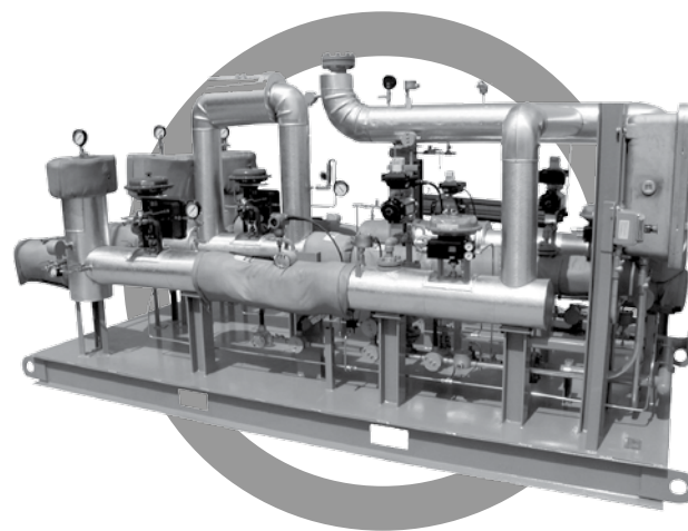
Tri-gas blending skid for testing turbine engines on off-spec. gases
