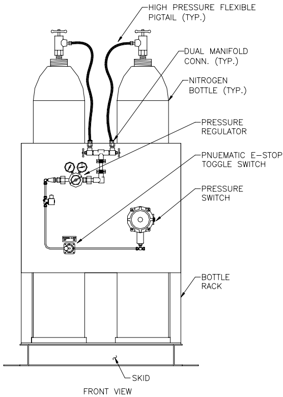
NITROGEN BANK LAYOUT
