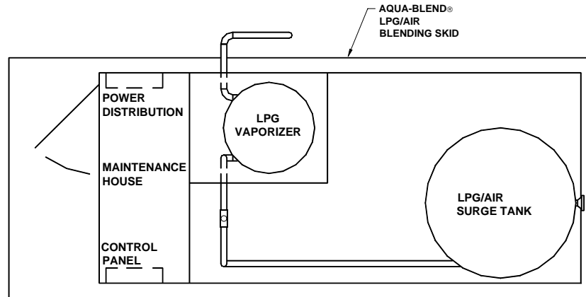
TYPICAL STANDBY SYSTEM
