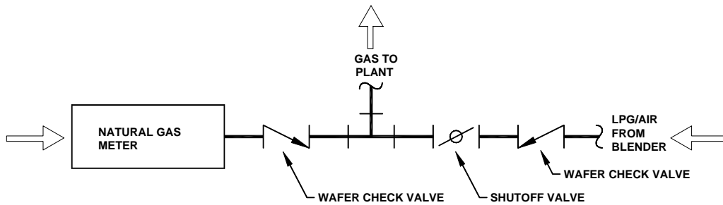
TYPICAL TIE-IN DETAIL
